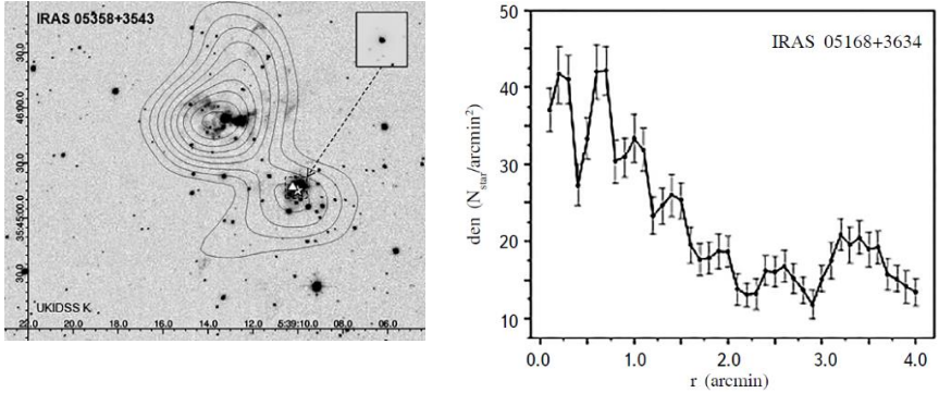
Figure 1. ( Left ) NIR images and isodensities of IRAS05358+3543 star-forming region. IRAS and MSX sources are indicated by stars and triangles, respectively. ( Right ) Radial distribution of the stellar density relative to IRAS05168+3634 source. Vertical lines are standard errors.
